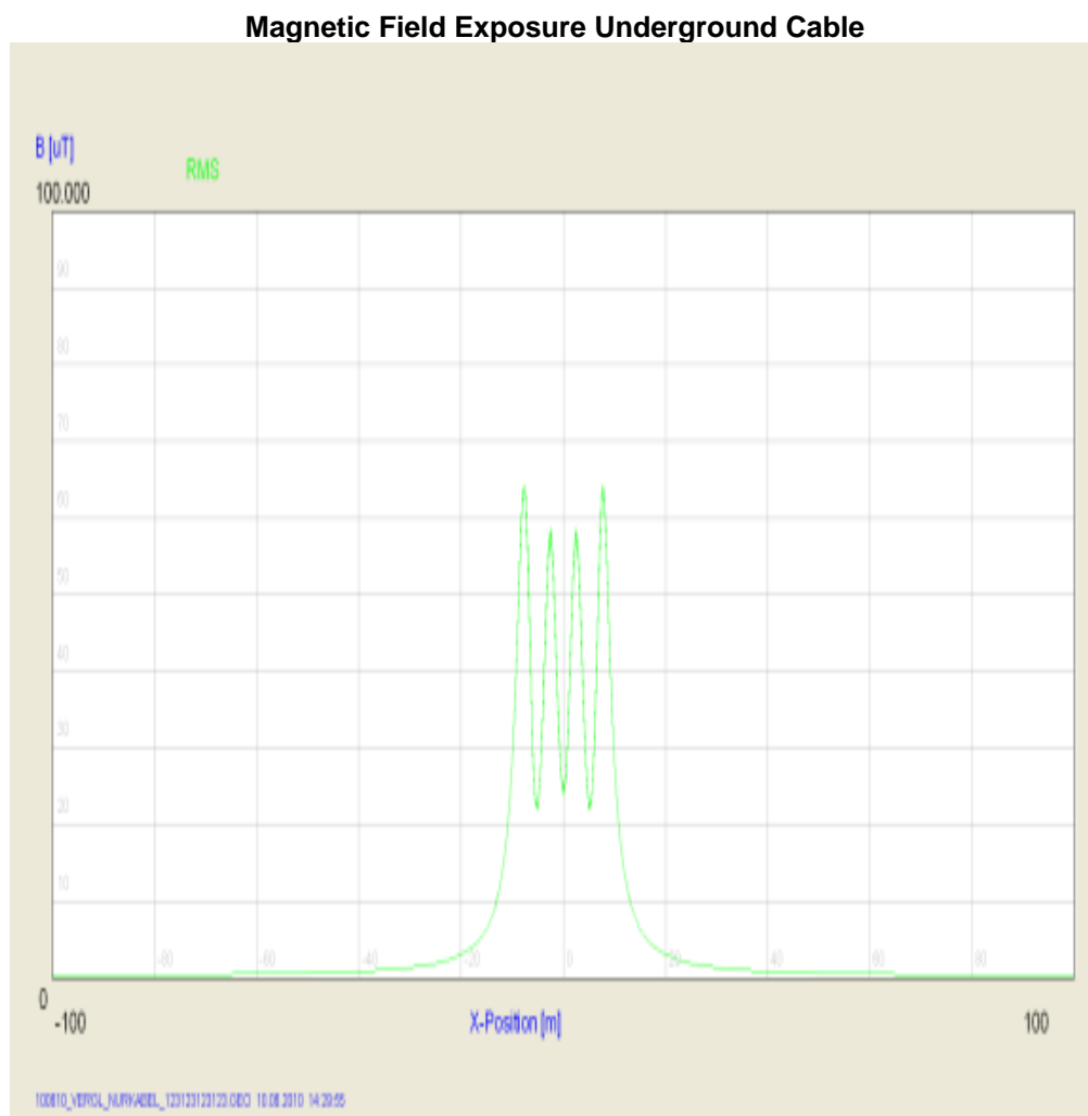
Figure 16: Magnetic Field Exposure UGC calculated at 20 cm above ground and at X meters from the centre of the cable circuit
